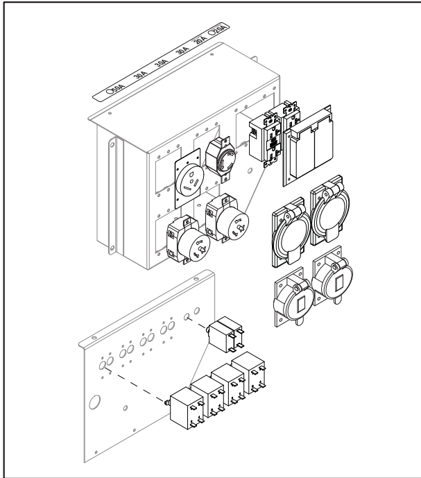
PART NUMBER 13540 Receptacle Panel (2x5-20R, 1xTT-30R, 1xL6-30R, 2x50A)
