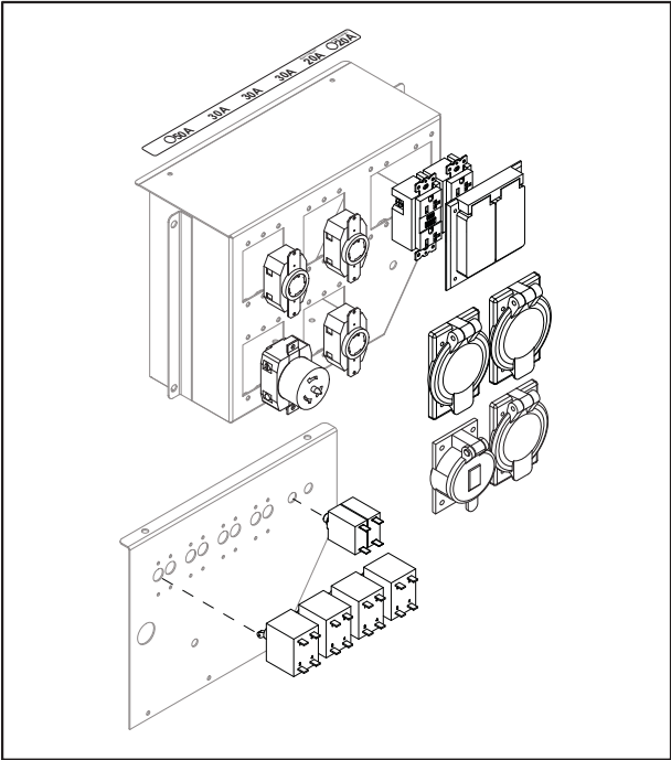
PART NUMBER 10395 Receptacle Panel (2x5-20R, 3xL14-30R, 1x50A)
