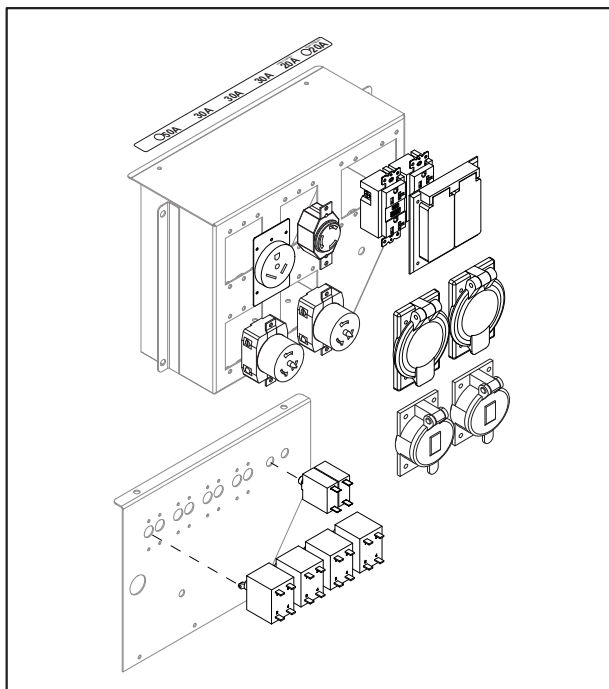
PART NUMBER 10398 Receptacle Panel (2x5-20R, 1xTT-30R, 1xL6-30R, 2x50A)
