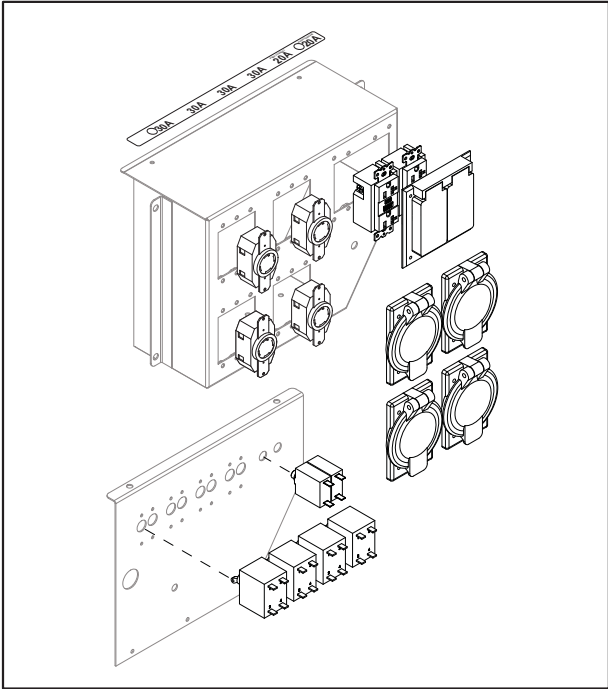
PART NUMBER 10396 Receptacle Panel (2x5-20R, 4xL14-30R)
