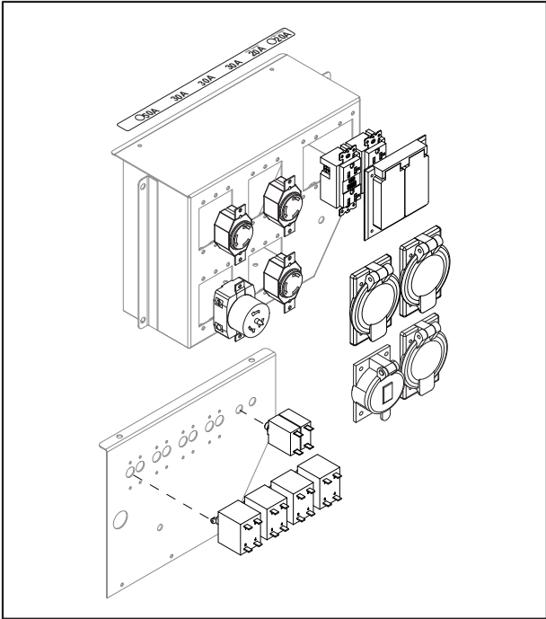
PART NUMBER 10394 Receptacle Panel (2x5-20R, 3xL6-30R, 1x50A)
