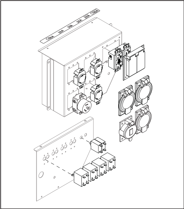
PART NUMBER 10397 Receptacle Panel (2x5-20R, 3xL6-20R, 1x50A)
